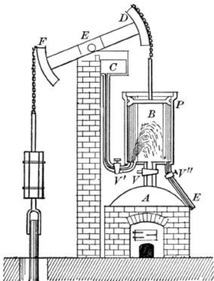
"Diagram of the Newcomen steam engine"
